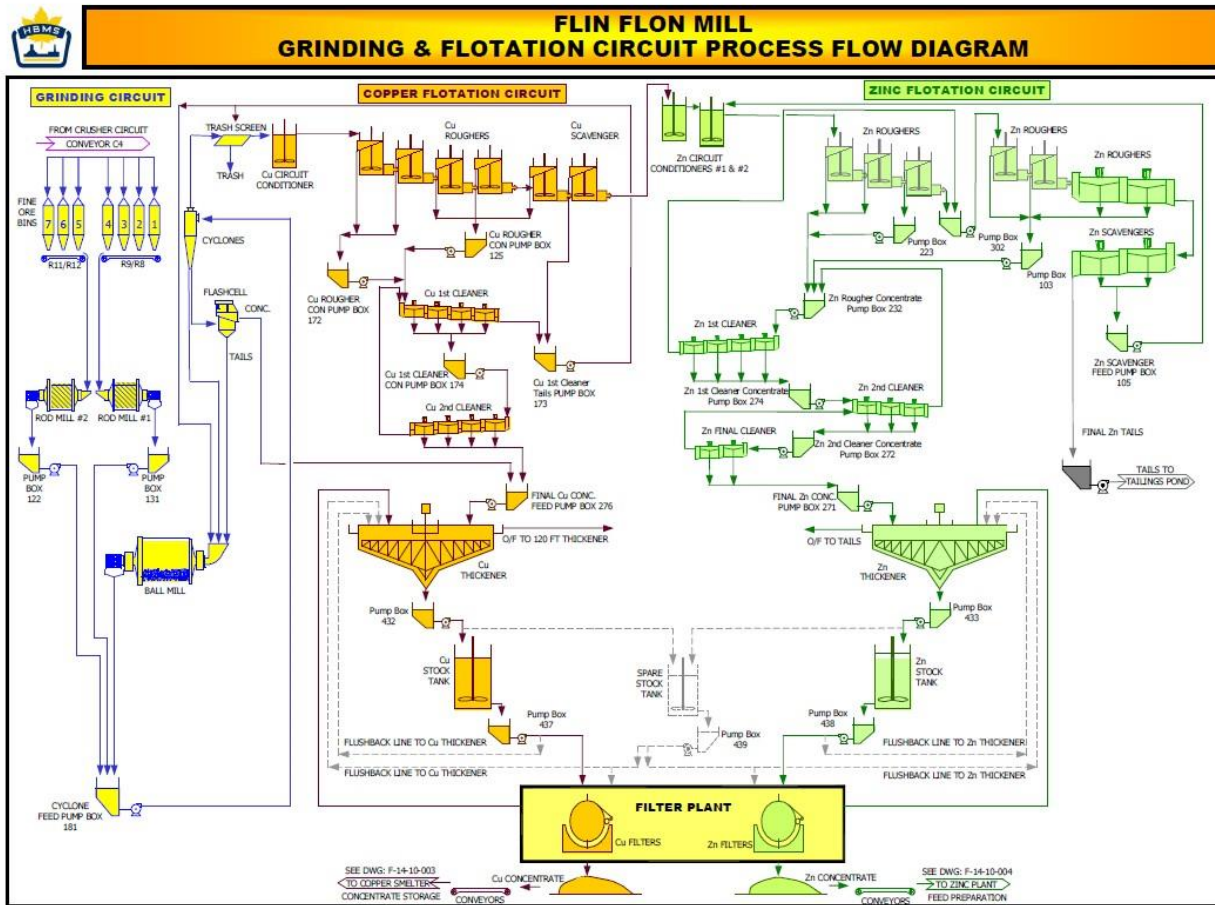
Figure 2: Flin Flon Concentrator Worksheet
