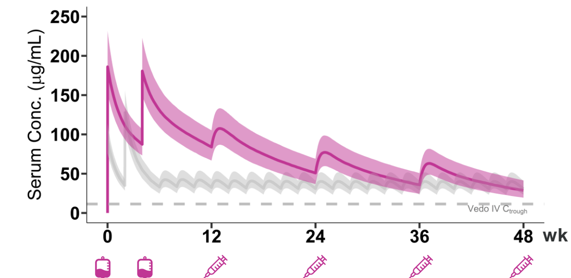
Figure 5: Simulated PK profiles of SPY001 (IV at W0, W4; SC at W12 and Q12W) and vedolizumab (IV at W0, W2; SC dose Q2W). Based on average t_{1/2} extension of ~3x with YTE and published human vedolizumab t_{1/2} of 25 days. Solid line: simulated median; Shaded area: interquartile range. Stochastic simulations: n=2,000 virtual subjects.
