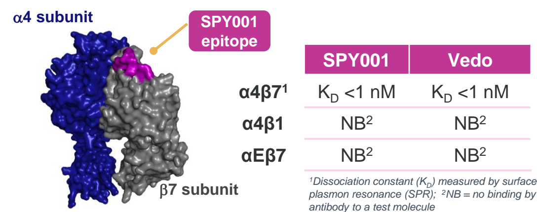
Figure 1: Predicted binding site for SPY001 (left); dissociation constants for SPY001 and vedolizumab (vedo) for \alpha4\beta7 and related integrins by surface plasmon resonance (right).
